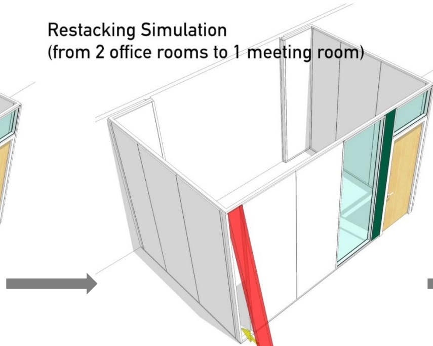
Restacking Simulation (from 2 office rooms to 1 meeting room)
